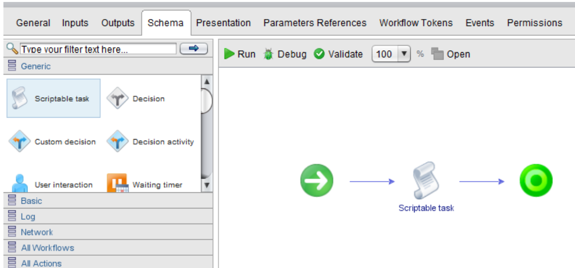
Slika 7.1 JavaScriptExample workflow
